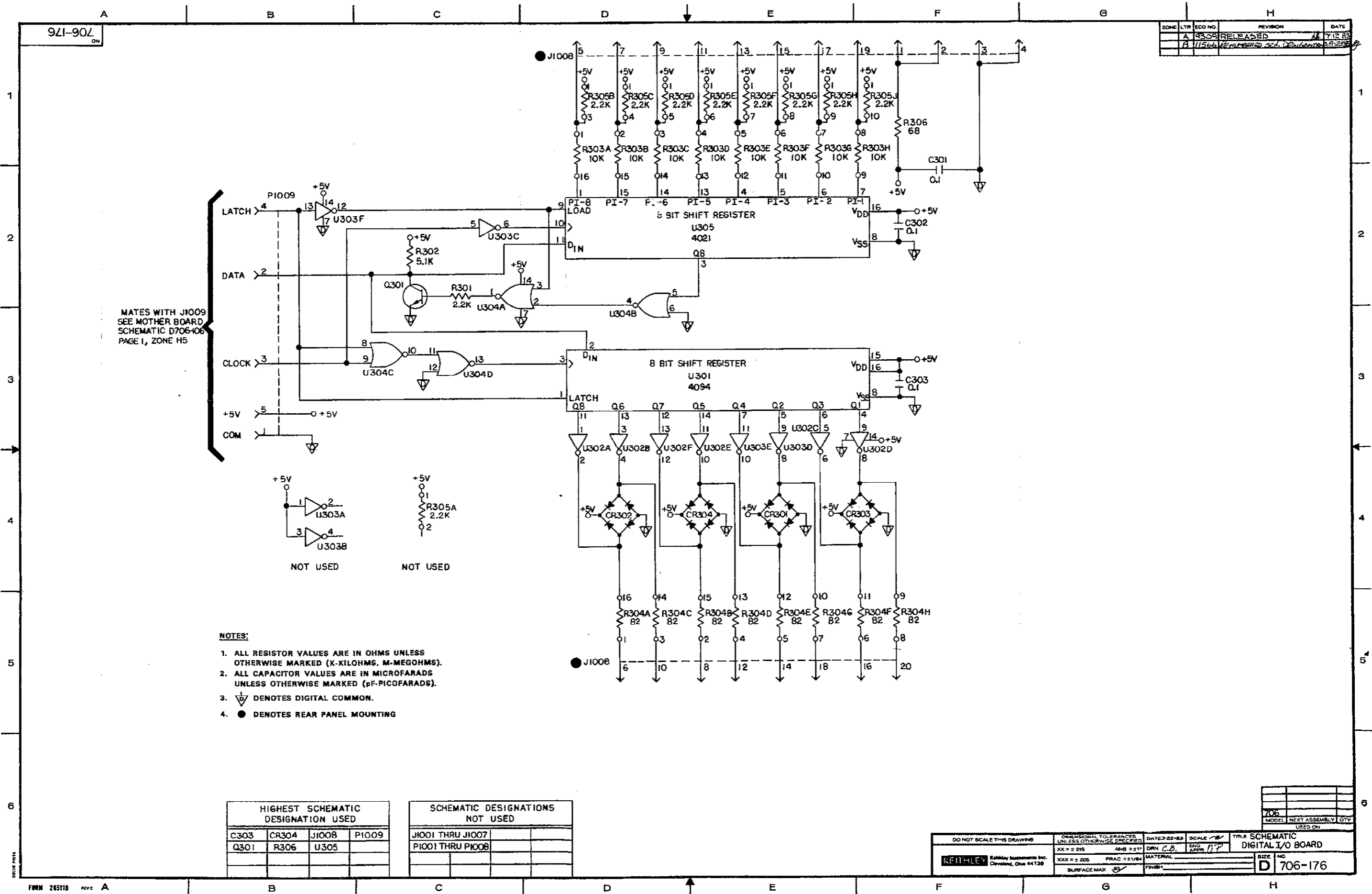
Figure 6-6. Digital I/O Board, Schematic Diagram, Dwg. No. 706-176
